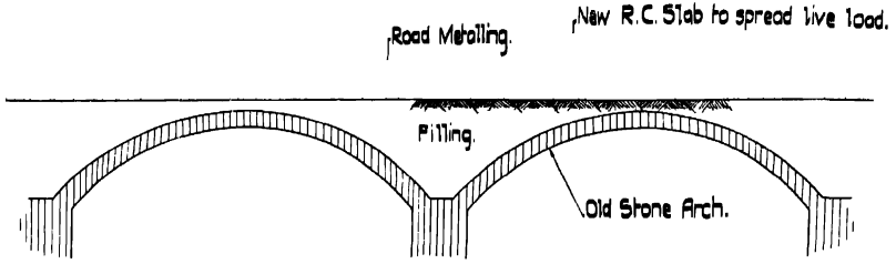
Fig. 211.—New Reinforced Concrete Slab spreading Live Loads and so relieving Old Arches.
